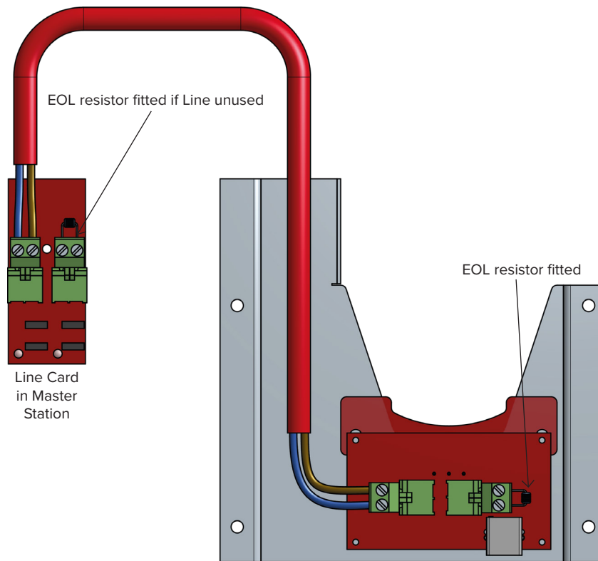
Figure 2: Type A Outstation Wiring Diagram
